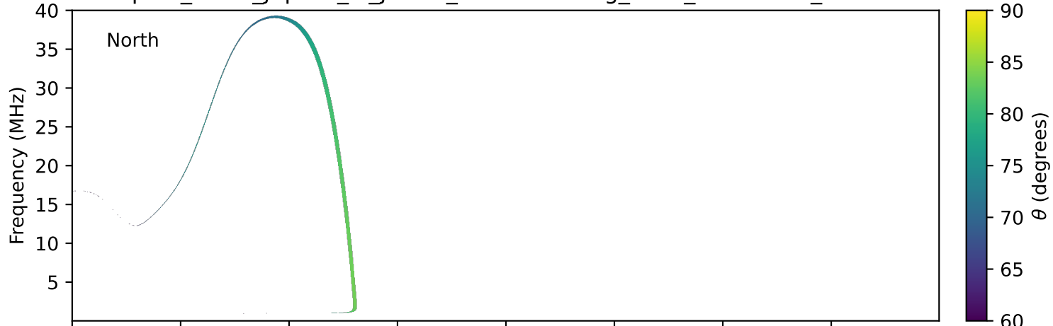
expres_earth_jupiter_io_jrm33_lossc-wid1deg_3kev_20020401_v11.cdf
