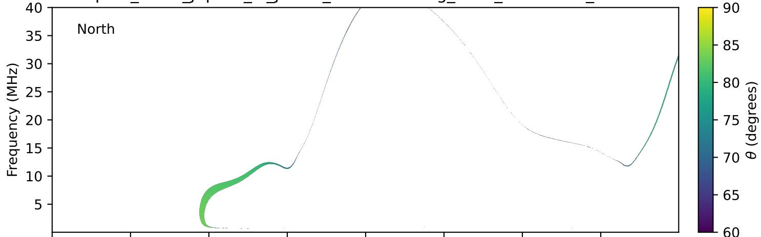
expres_earth_jupiter_io_jrm09_lossc-wid1deg_3kev_20020425_v11.cdf
