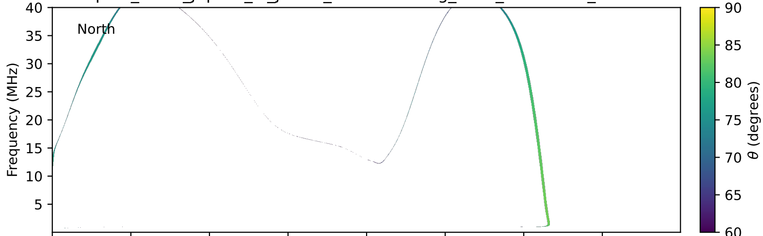
expres_earth_jupiter_io_jrm09_lossc-wid1deg_3kev_20020420_v11.cdf
