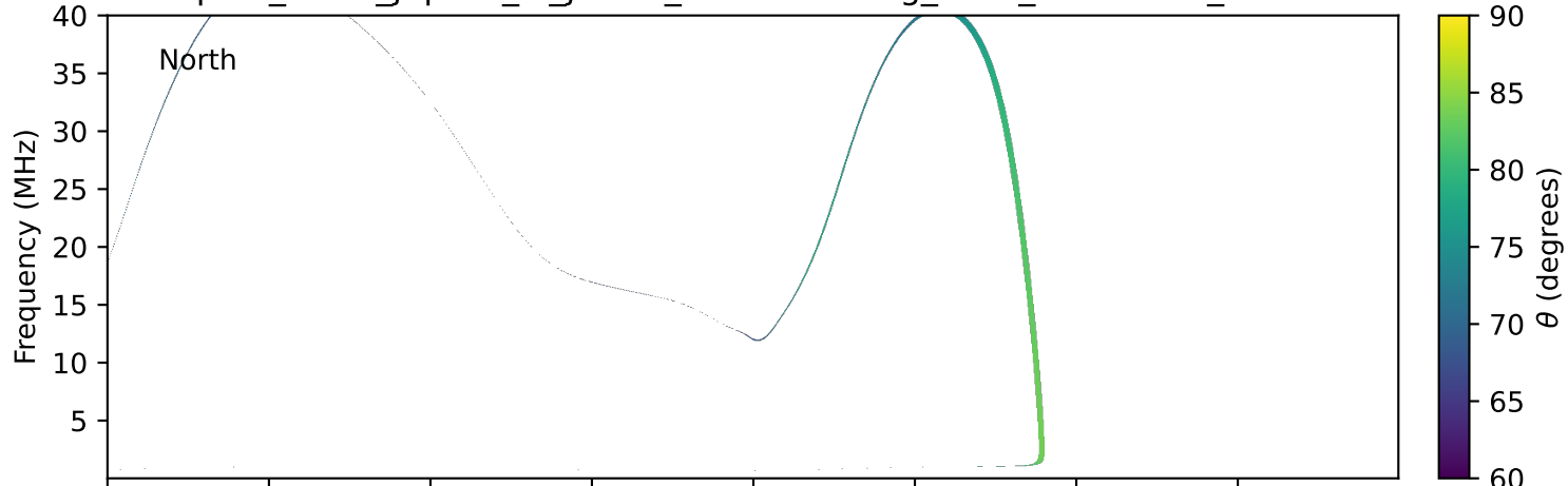
expres_earth_jupiter_io_jrm09_lossc-wid1deg_3kev_20020413_v11.cdf
