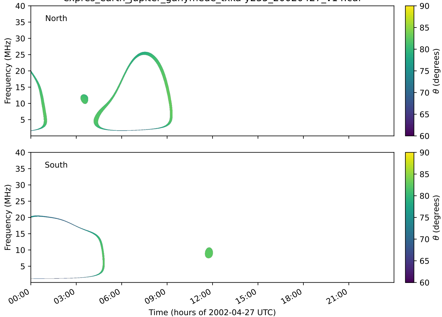
expres_earth_jupiter_ganymede_txka-y235_20020427_v14.cdf
