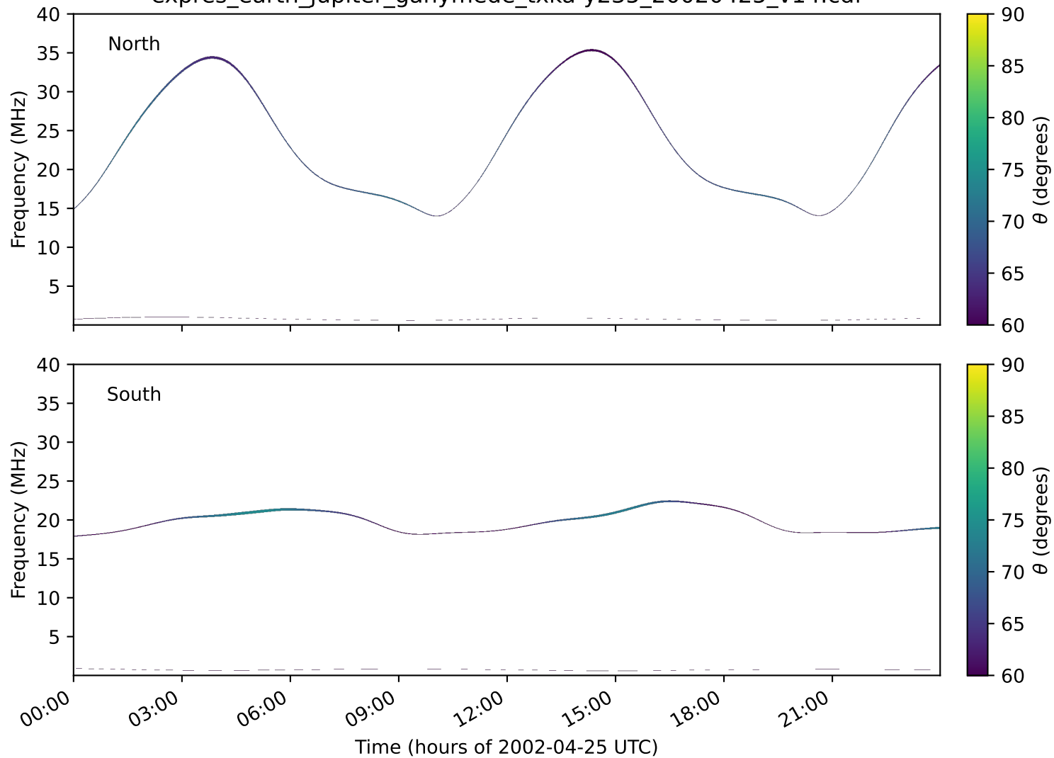
expres_earth_jupiter_ganymede_txka-y235_20020425_v14.cdf
