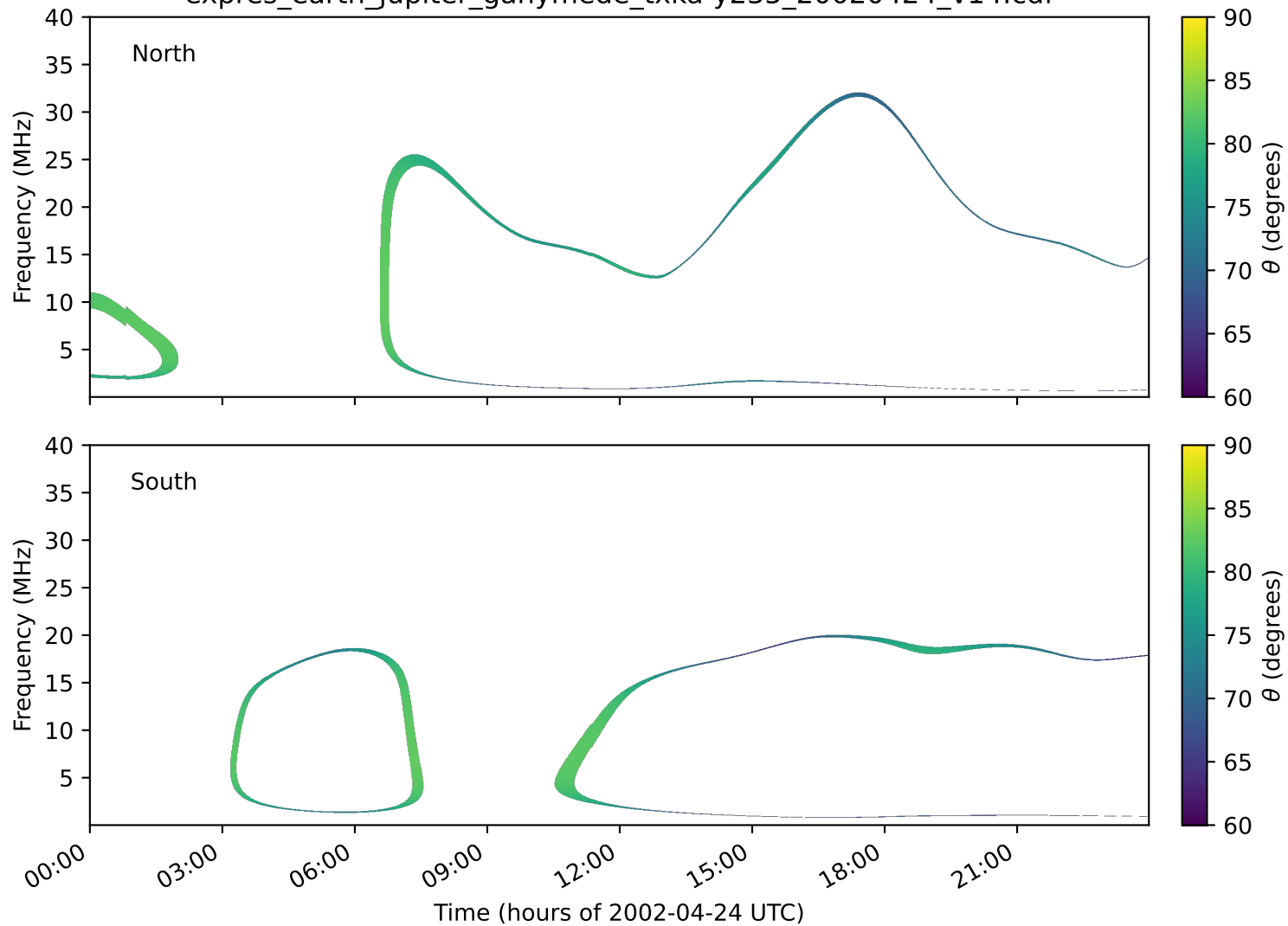
expres_earth_jupiter_ganymede_txka-y235_20020424_v14.cdf
