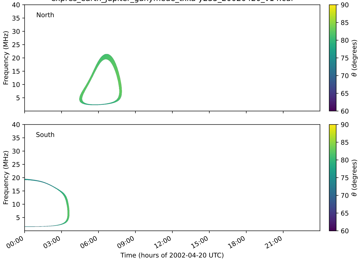
expres_earth_jupiter_ganymede_txka-y235_20020420_v14.cdf
