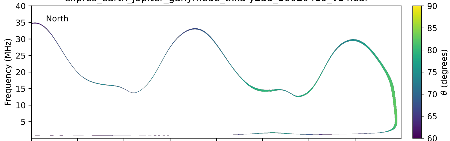
expres_earth_jupiter_ganymede_txka-y235_20020419_v14.cdf
