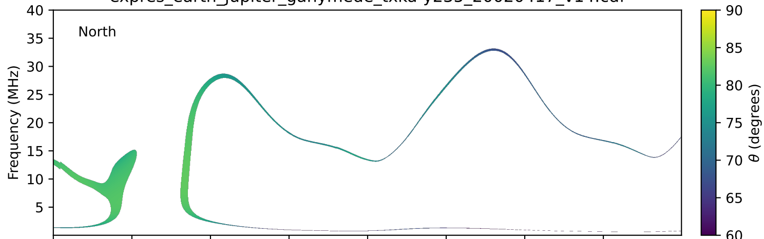
expres_earth_jupiter_ganymede_txka-y235_20020417_v14.cdf
