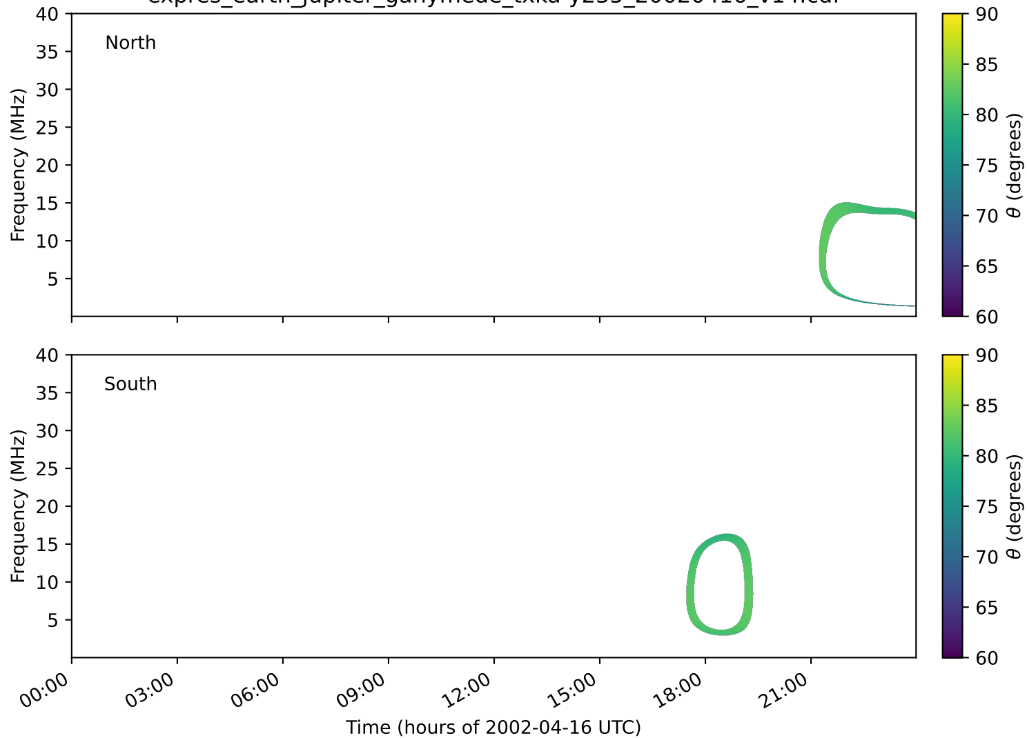
expres_earth_jupiter_ganymede_txka-y235_20020416_v14.cdf
