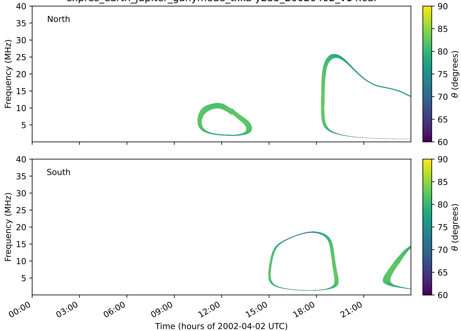
expres_earth_jupiter_ganymede_txka-y235_20020402_v14.cdf
