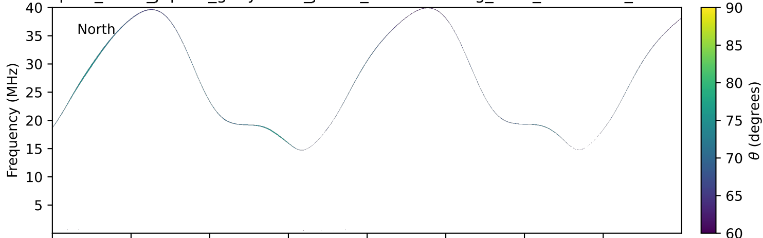
expres_earth_jupiter_ganymede_jrm33_lossc-wid1deg_3kev_20020425_v11.cdf
