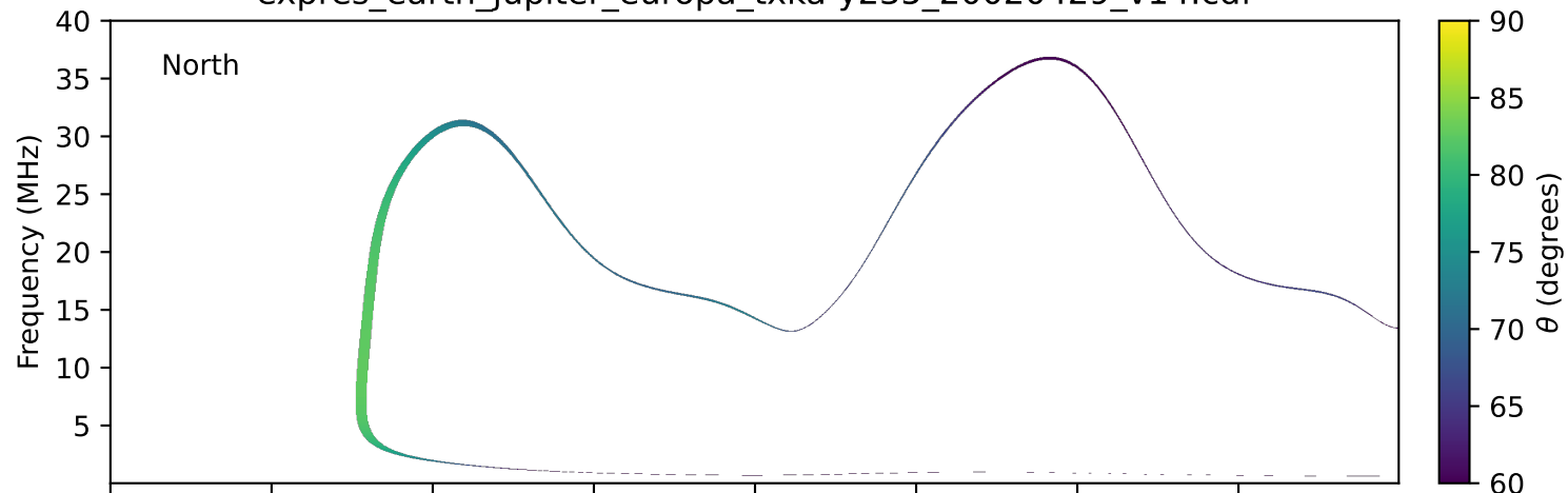
expres_earth_jupiter_europa_txka-y235_20020429_v14.cdf
