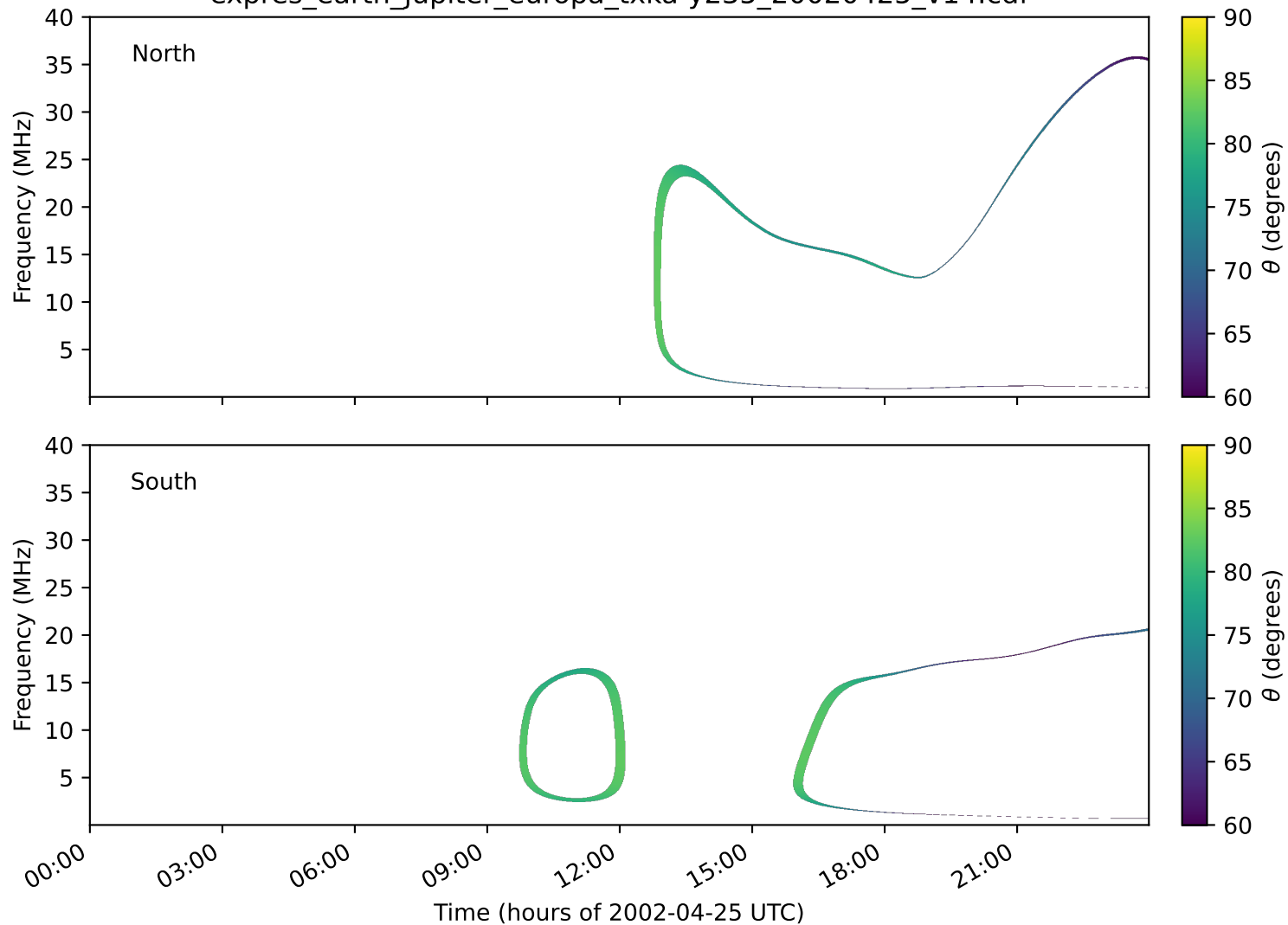
expres_earth_jupiter_europa_txka-y235_20020425_v14.cdf
