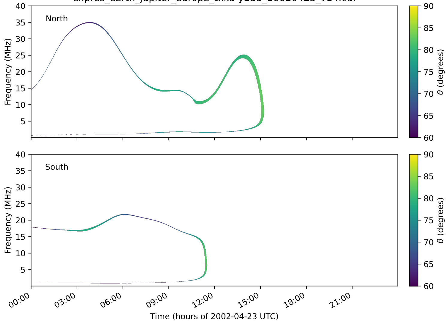
expres_earth_jupiter_europa_txka-y235_20020423_v14.cdf
