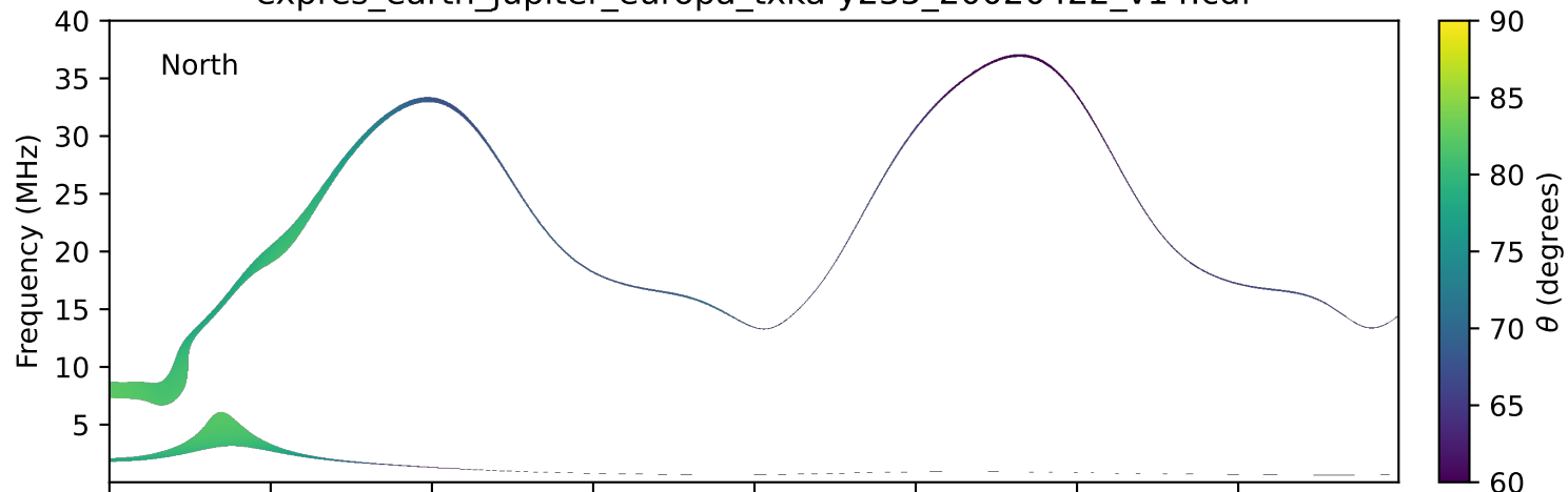
expres_earth_jupiter_europa_txka-y235_20020422_v14.cdf
