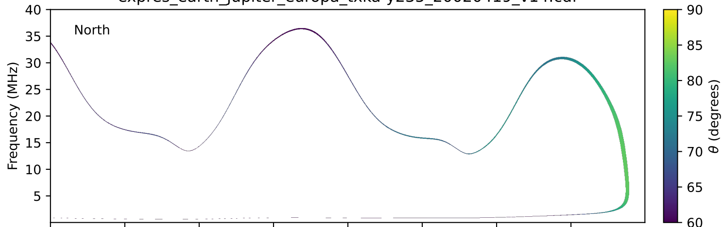
expres_earth_jupiter_europa_txka-y235_20020419_v14.cdf
