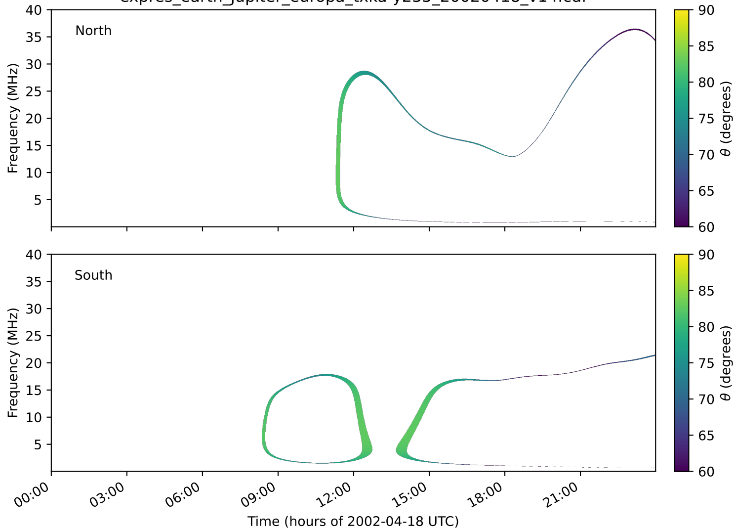
expres_earth_jupiter_europa_txka-y235_20020418_v14.cdf
