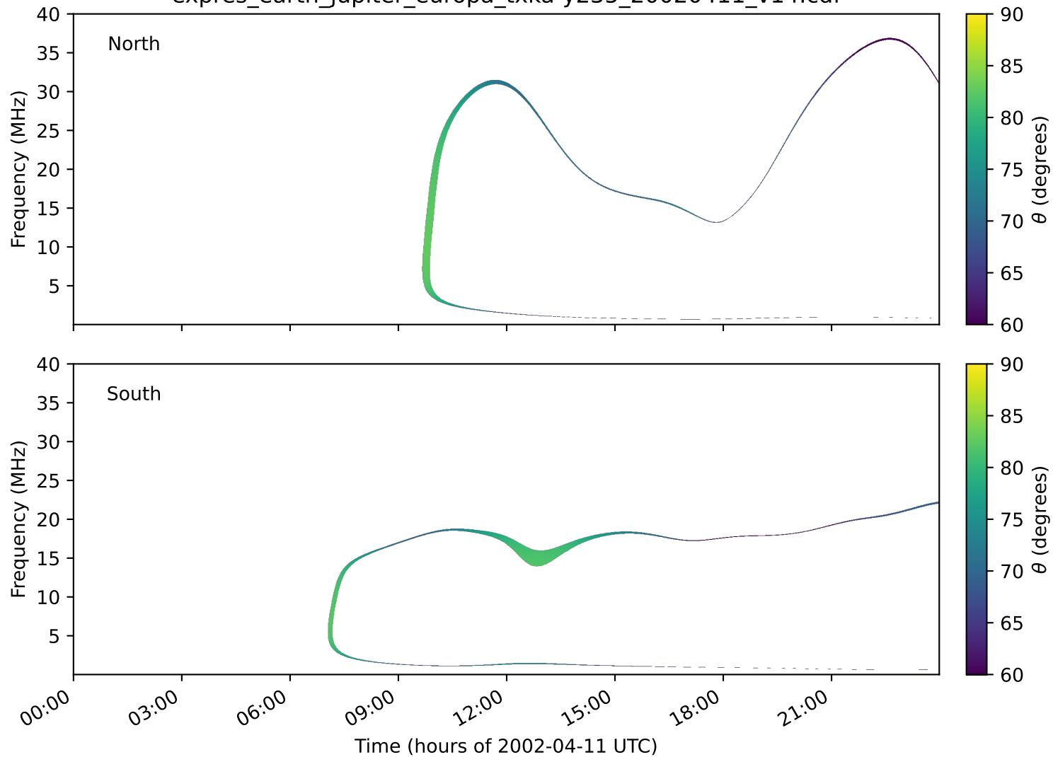
expres_earth_jupiter_europa_txka-y235_20020411_v14.cdf
