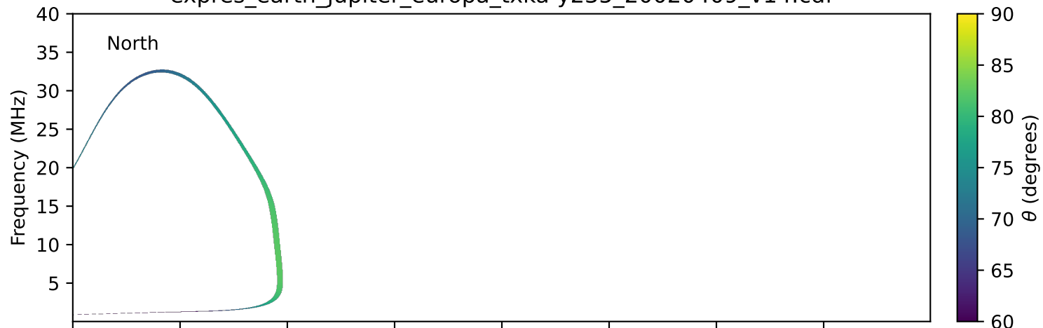
expres_earth_jupiter_europa_txka-y235_20020409_v14.cdf
