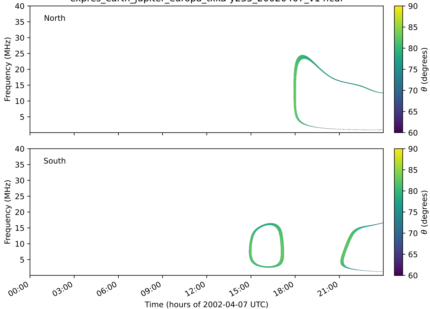
expres_earth_jupiter_europa_txka-y235_20020407_v14.cdf
