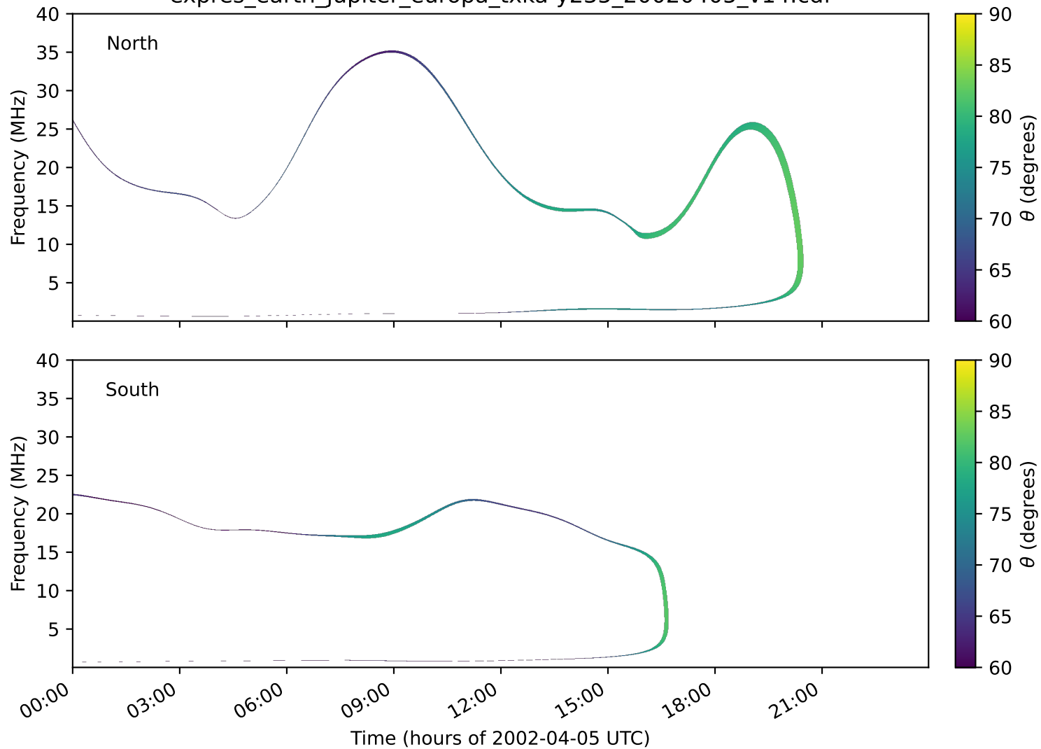
expres_earth_jupiter_europa_txka-y235_20020405_v14.cdf
