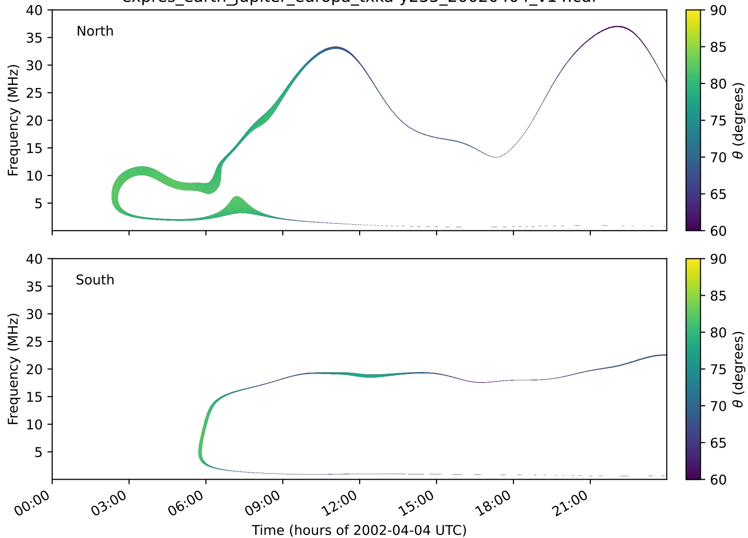
expres_earth_jupiter_europa_txka-y235_20020404_v14.cdf
