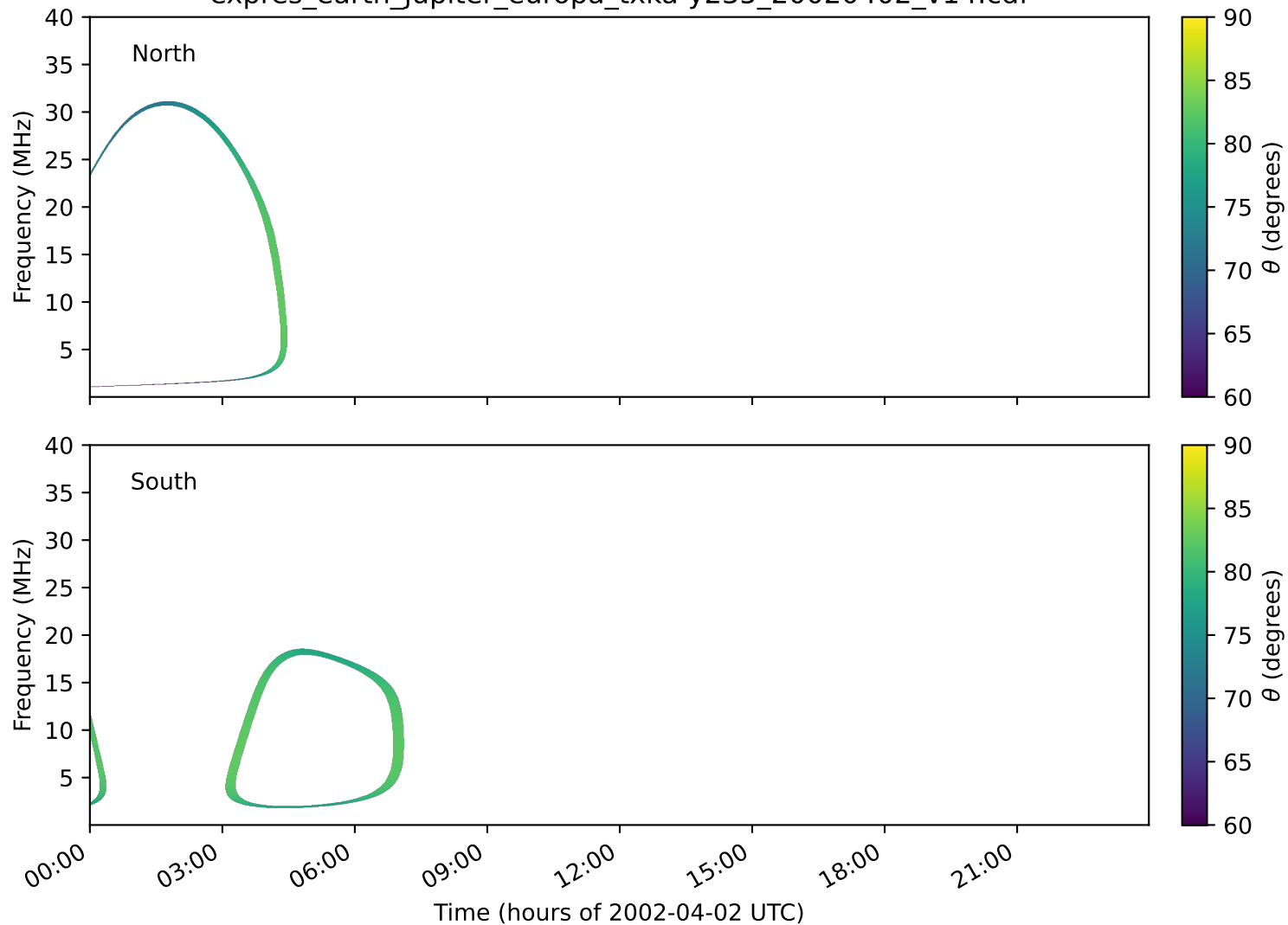
expres_earth_jupiter_europa_txka-y235_20020402_v14.cdf
