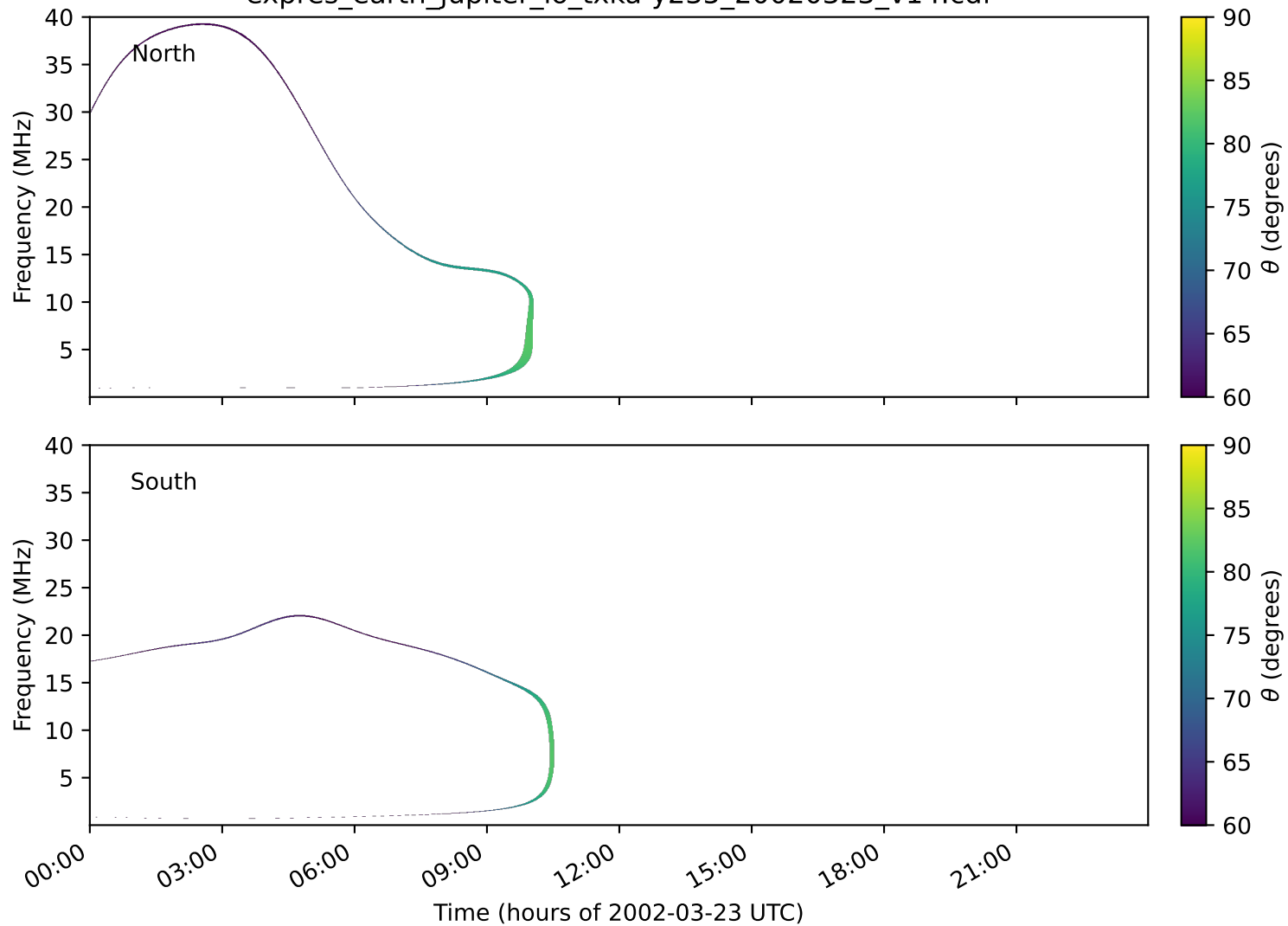
expres_earth_jupiter_io_txka-y235_20020323_v14.cdf
