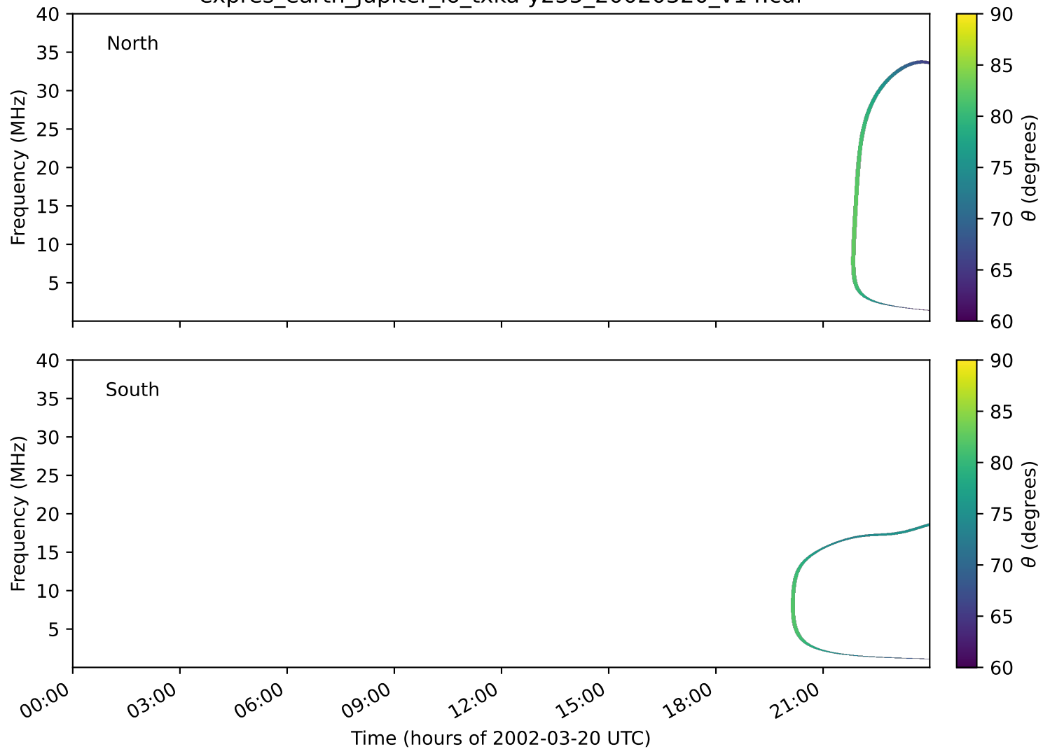
expres_earth_jupiter_io_txka-y235_20020320_v14.cdf
