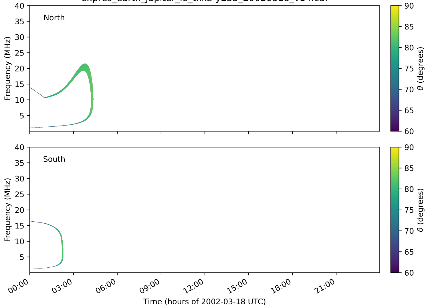
expres_earth_jupiter_io_txka-y235_20020318_v14.cdf
