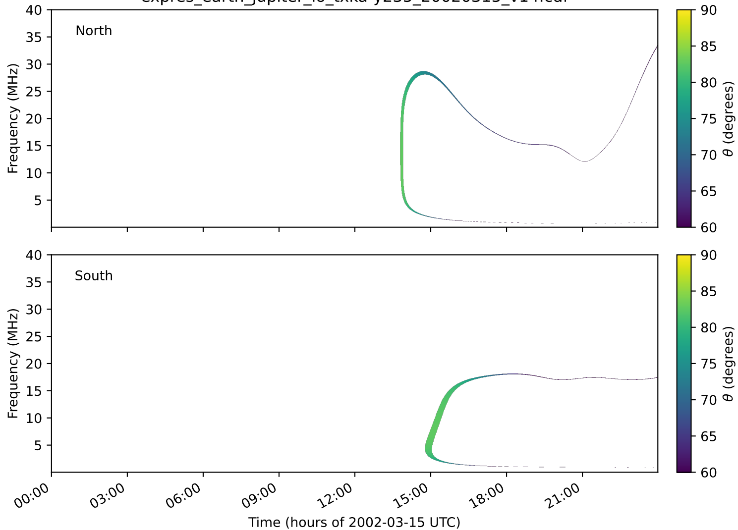
expres_earth_jupiter_io_txka-y235_20020315_v14.cdf
