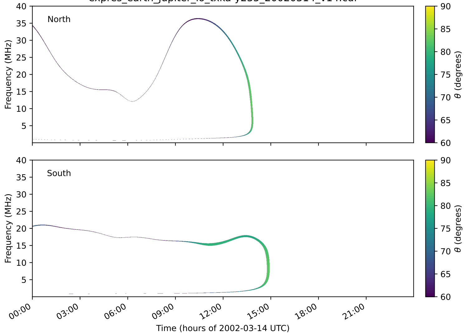
expres_earth_jupiter_io_txka-y235_20020314_v14.cdf
