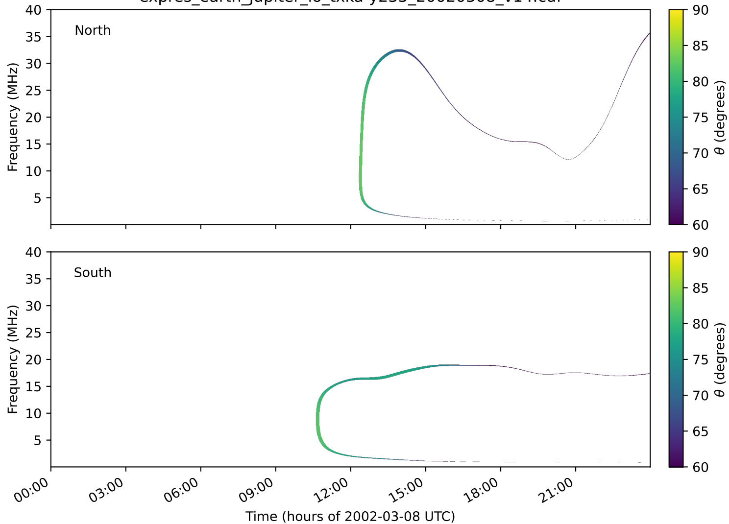
expres_earth_jupiter_io_txka-y235_20020308_v14.cdf
