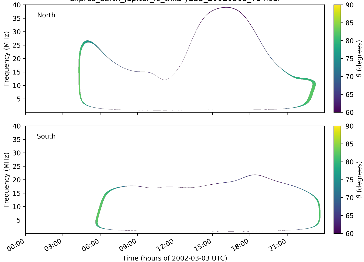
expres_earth_jupiter_io_txka-y235_20020303_v14.cdf
