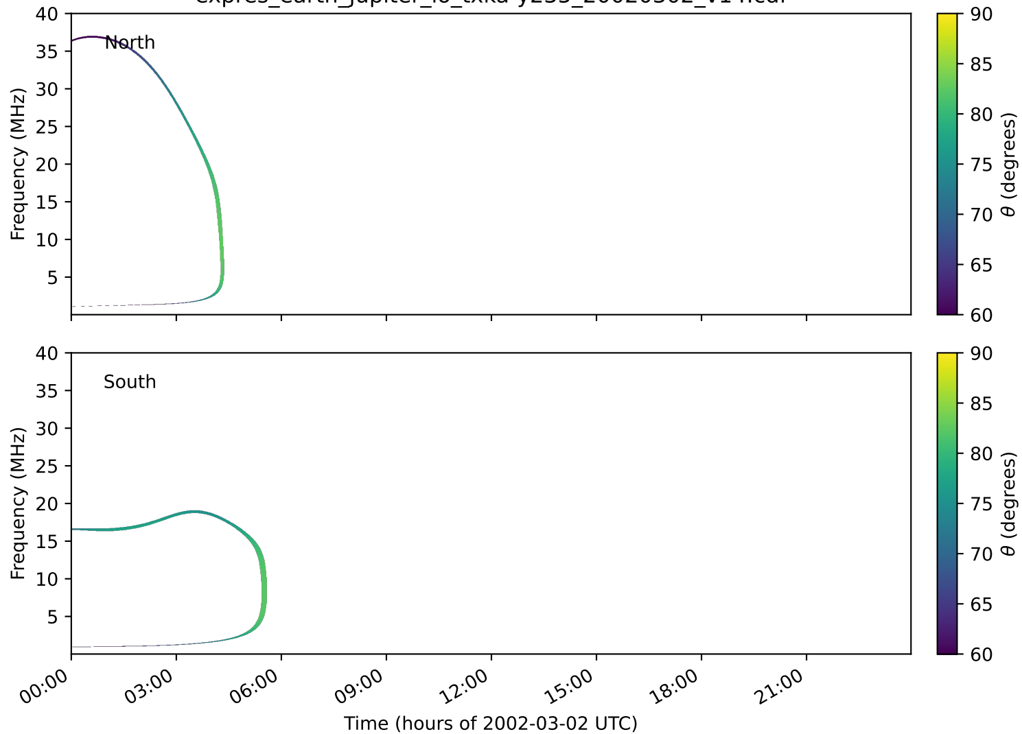
expres_earth_jupiter_io_txka-y235_20020302_v14.cdf
