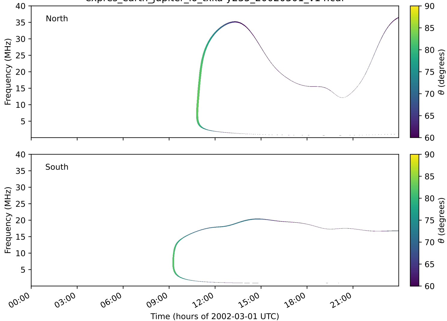
expres_earth_jupiter_io_txka-y235_20020301_v14.cdf
