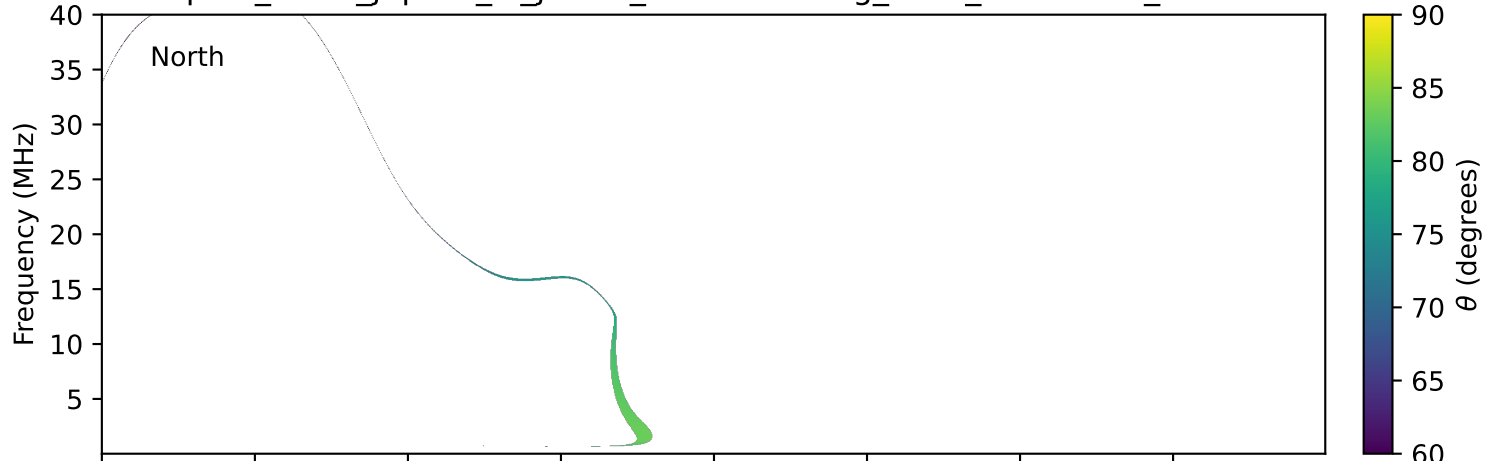
expres_earth_jupiter_io_jrm33_lossc-wid1deg_3kev_20020323_v11.cdf
