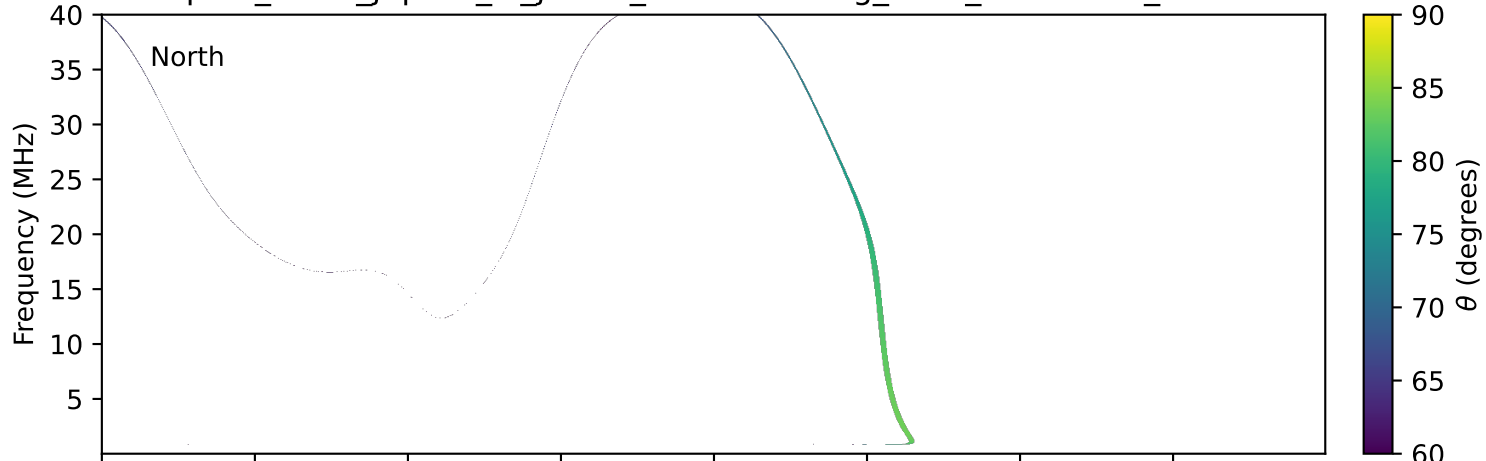
expres_earth_jupiter_io_jrm33_lossc-wid1deg_3kev_20020321_v11.cdf
