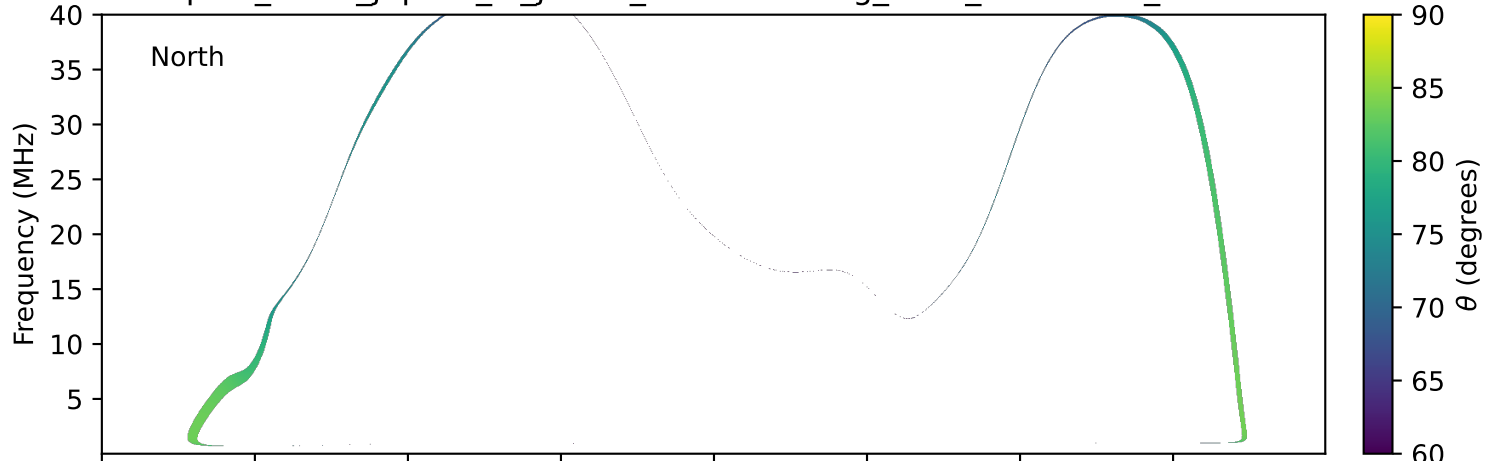
expres_earth_jupiter_io_jrm33_lossc-wid1deg_3kev_20020319_v11.cdf
