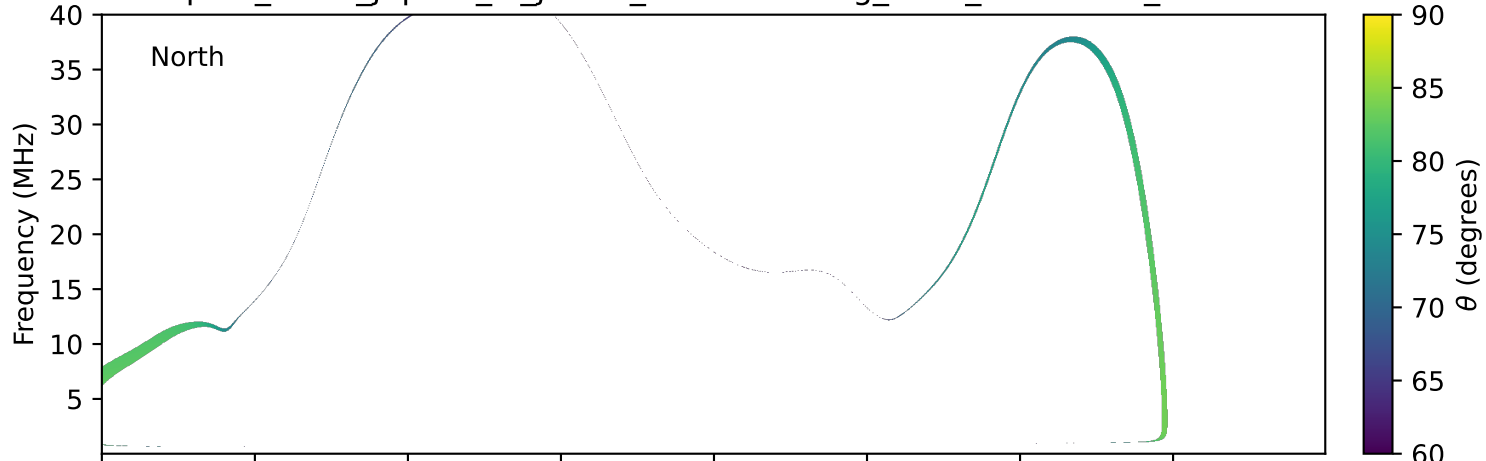
expres_earth_jupiter_io_jrm33_lossc-wid1deg_3kev_20020312_v11.cdf
