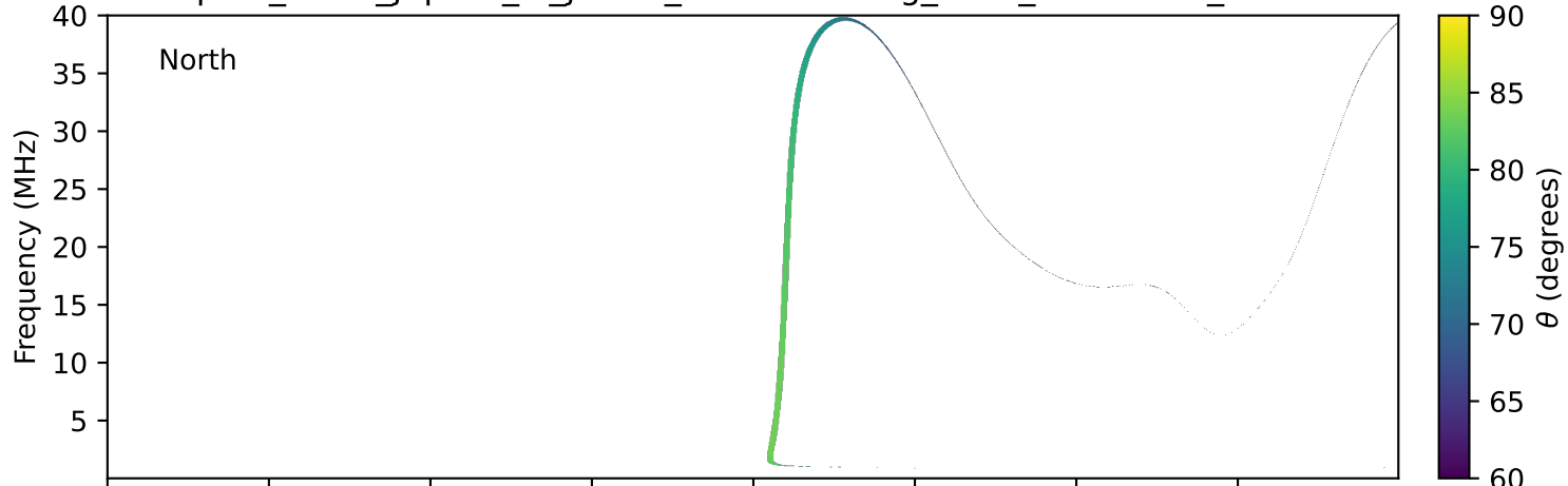
expres_earth_jupiter_io_jrm33_lossc-wid1deg_3kev_20020308_v11.cdf
