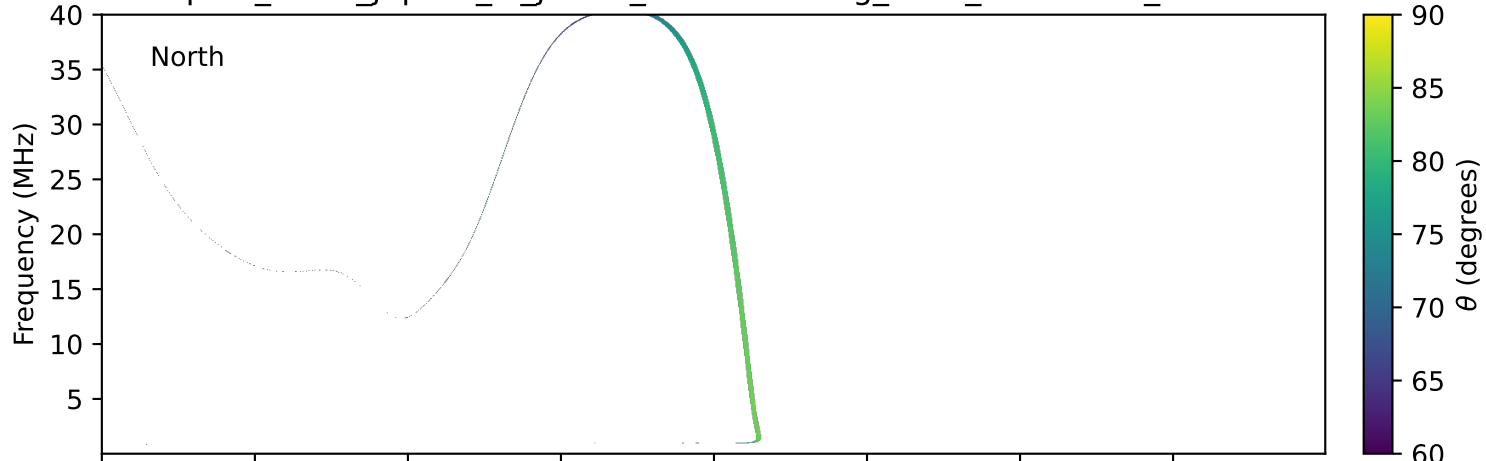
expres_earth_jupiter_io_jrm33_lossc-wid1deg_3kev_20020307_v11.cdf
