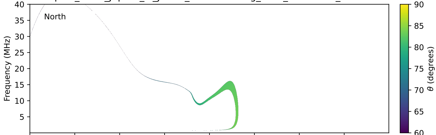
expres_earth_jupiter_io_jrm09_lossc-wid1deg_3kev_20020330_v11.cdf
