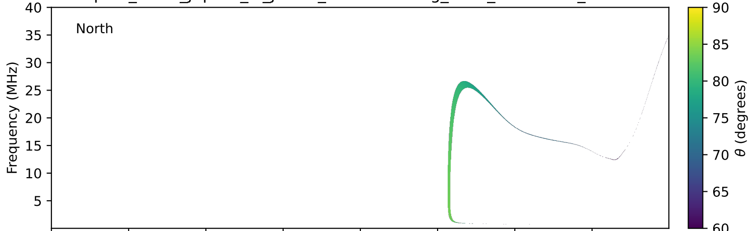
expres_earth_jupiter_io_jrm09_lossc-wid1deg_3kev_20020322_v11.cdf
