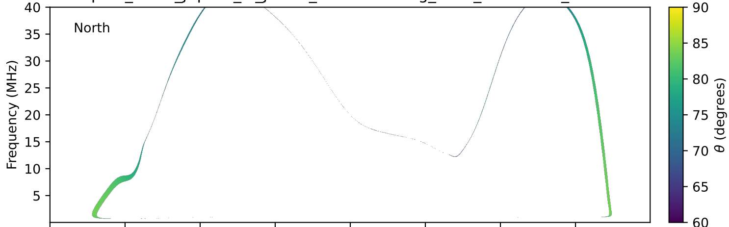
expres_earth_jupiter_io_jrm09_lossc-wid1deg_3kev_20020319_v11.cdf
