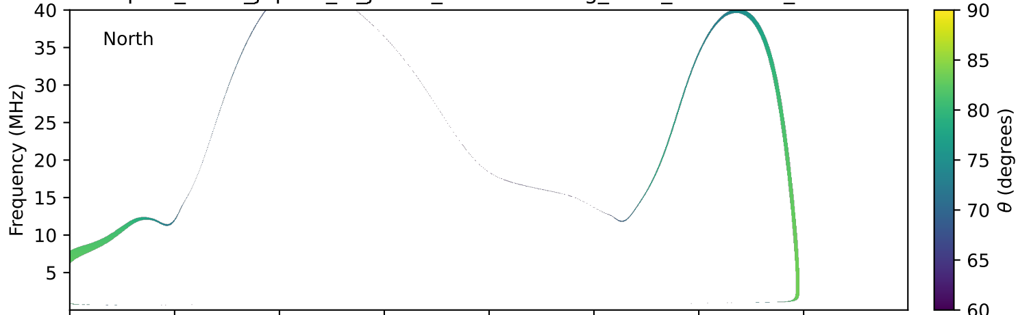
expres_earth_jupiter_io_jrm09_lossc-wid1deg_3kev_20020312_v11.cdf
