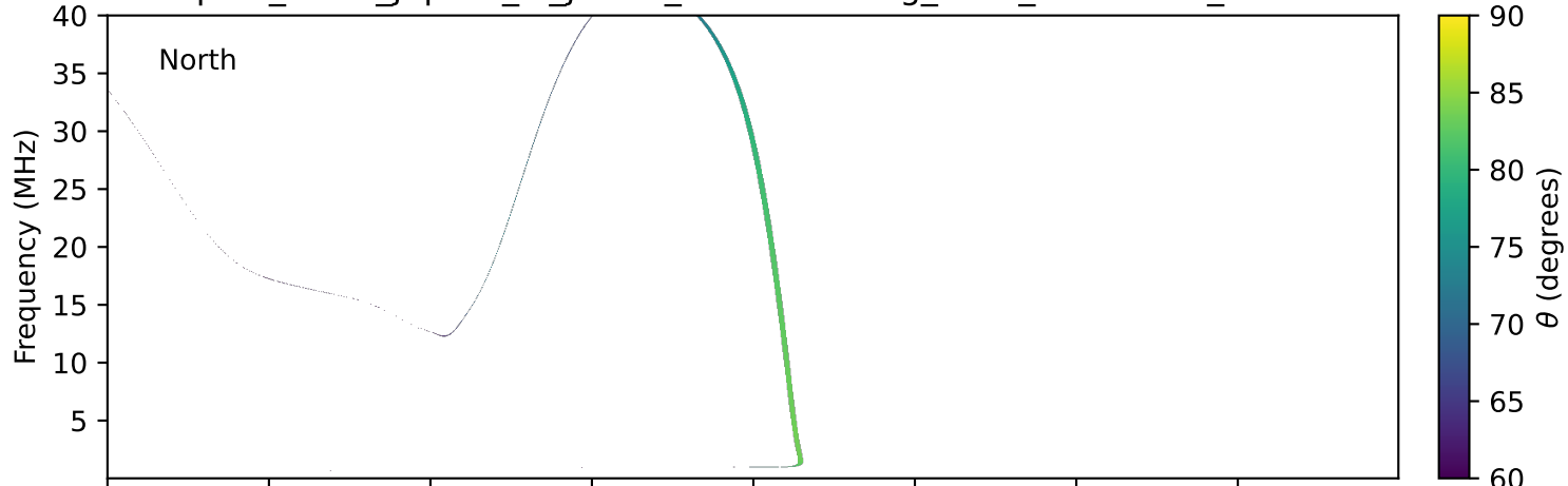
expres_earth_jupiter_io_jrm09_lossc-wid1deg_3kev_20020307_v11.cdf
