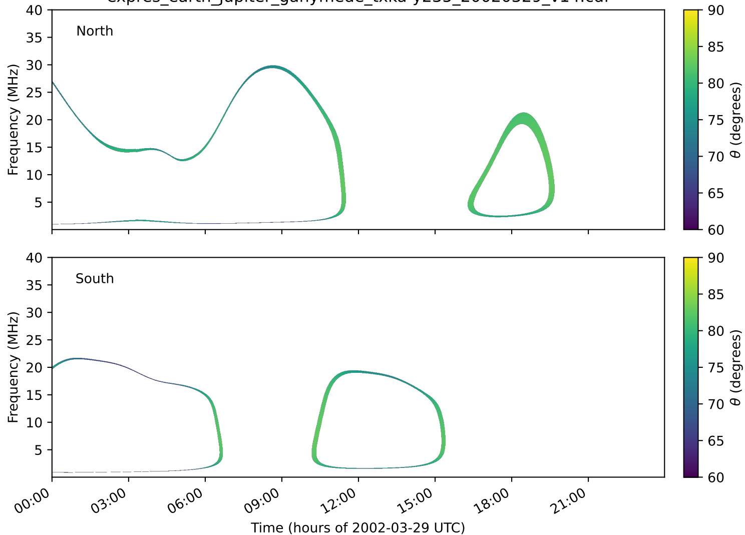
expres_earth_jupiter_ganymede_txka-y235_20020329_v14.cdf
