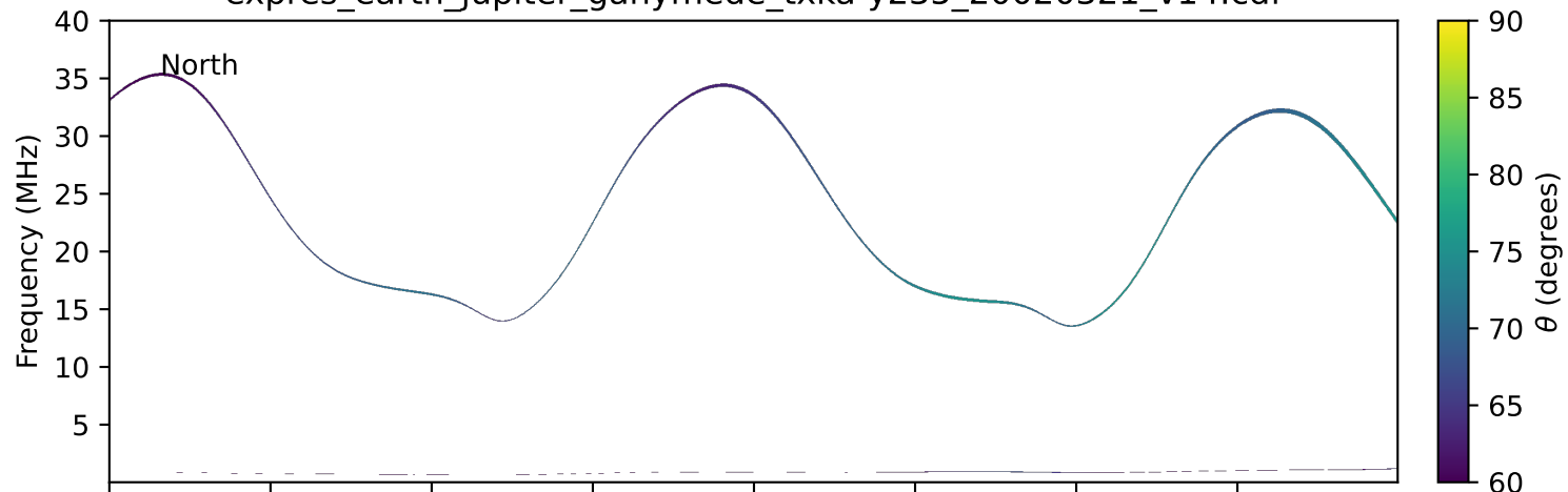
expres_earth_jupiter_ganymede_txka-y235_20020321_v14.cdf
