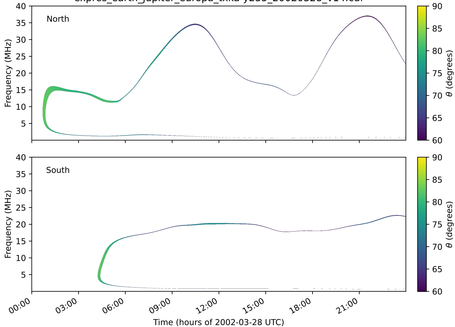
expres_earth_jupiter_europa_txka-y235_20020328_v14.cdf
