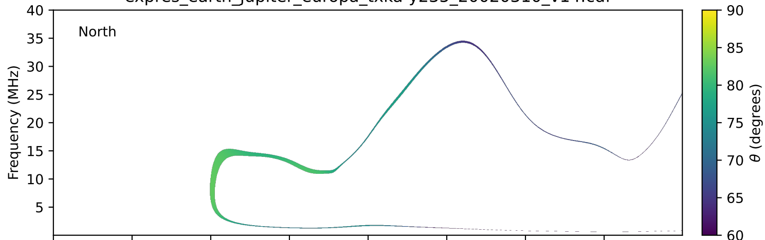
expres_earth_jupiter_europa_txka-y235_20020310_v14.cdf
