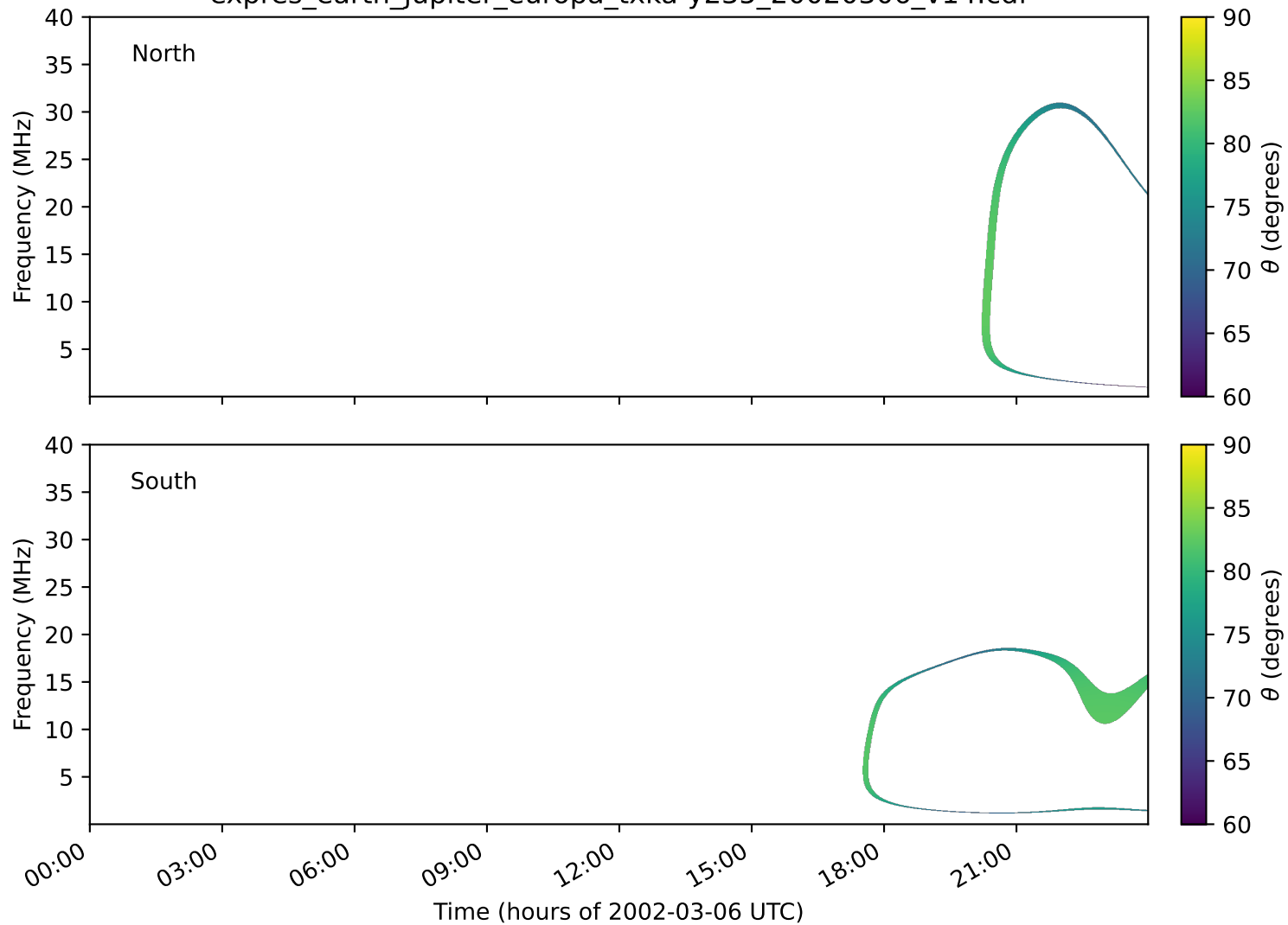
expres_earth_jupiter_europa_txka-y235_20020306_v14.cdf
